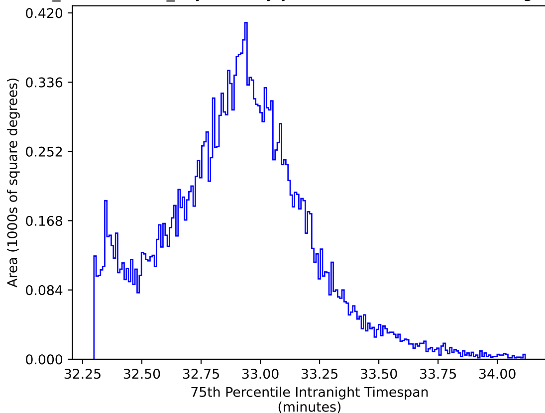
weather_cloudso2v3.4_10yrs All sky y band: 75th Percentile Intranight Timespan
