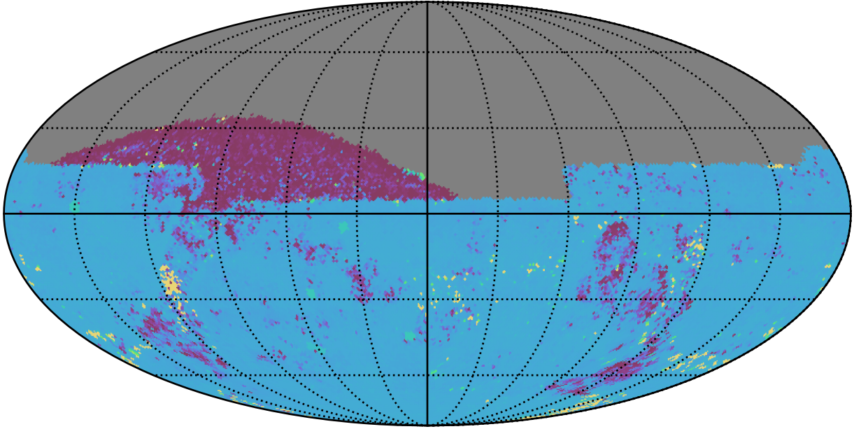
weather_cloudso2v3.4_10yrs All sky ug bands: 75th Percentile Intranight Timespan
