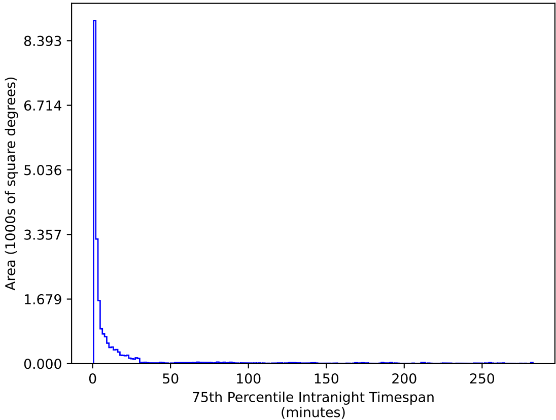
weather_cloudso2v3.4_10yrs All sky u band: 75th Percentile Intranight Timespan
