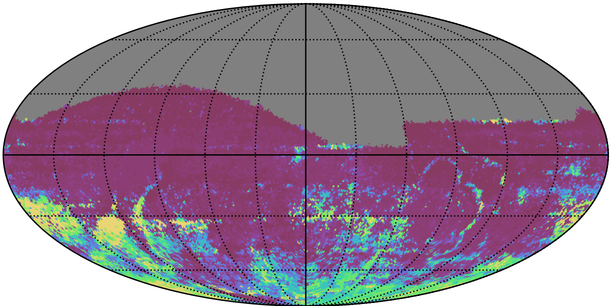
weather_cloudso2v3.4_10yrs All sky r band: 75th Percentile Intranight Timespan
