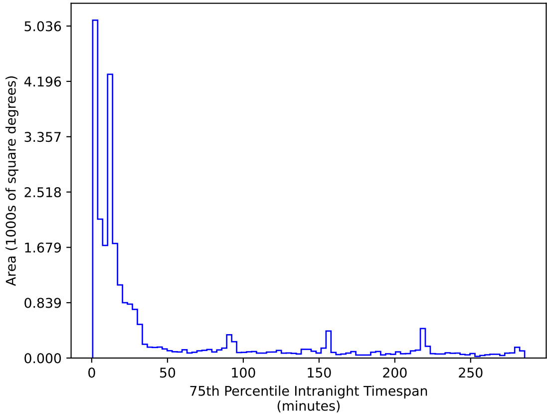
weather_cloudso2v3.4_10yrs All sky r band: 75th Percentile Intranight Timespan
