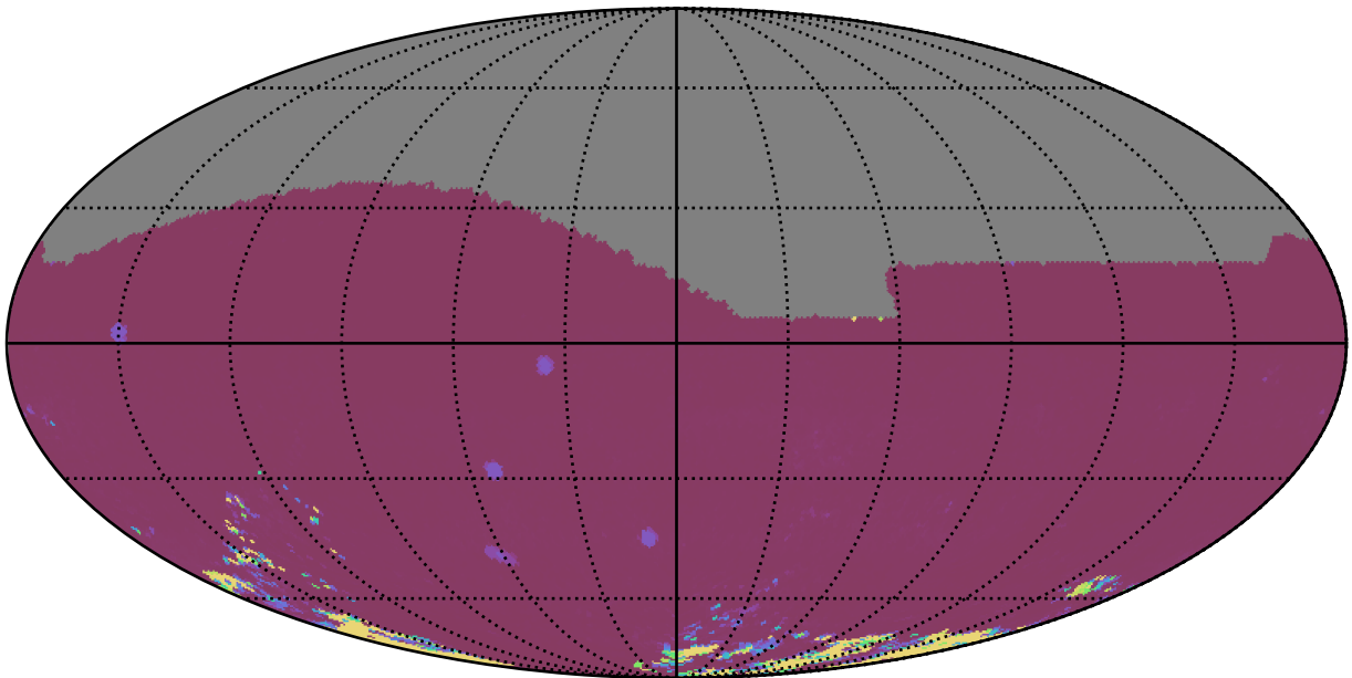
weather_cloudso2v3.4_10yrs All sky iz bands: 75th Percentile Intranight Timespan
