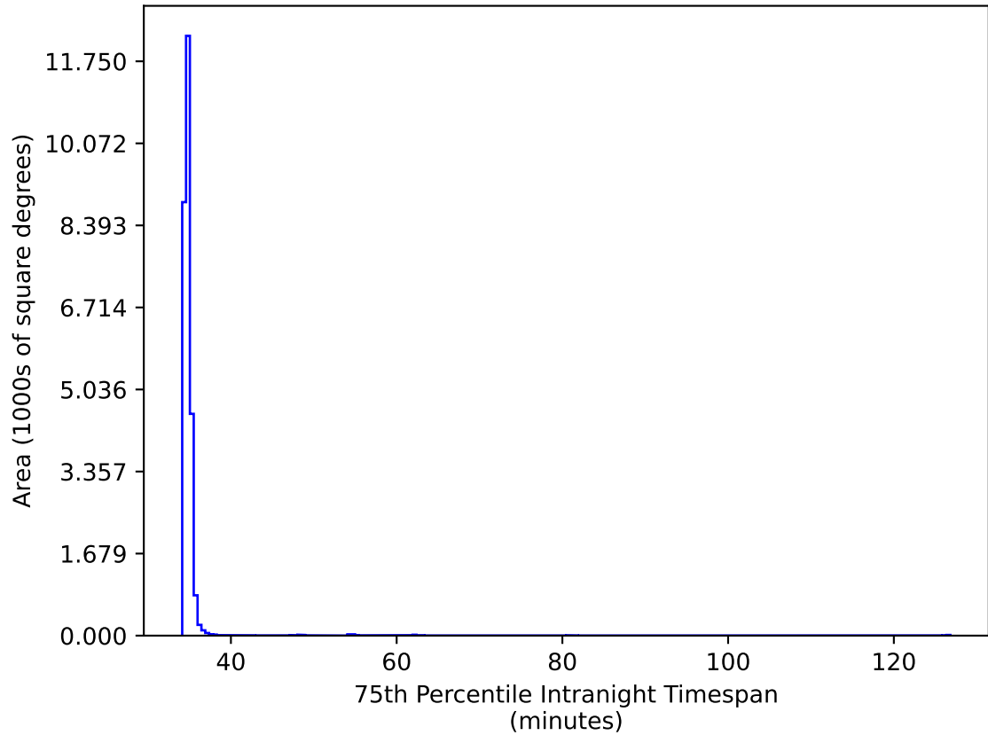
weather_cloudso2v3.4_10yrs All sky iz bands: 75th Percentile Intranight Timespan
