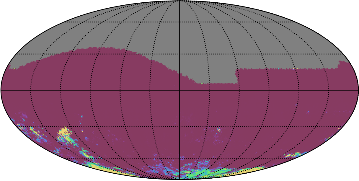
weather_cloudso2v3.4_10yrs All sky gr bands: 75th Percentile Intranight Timespan
