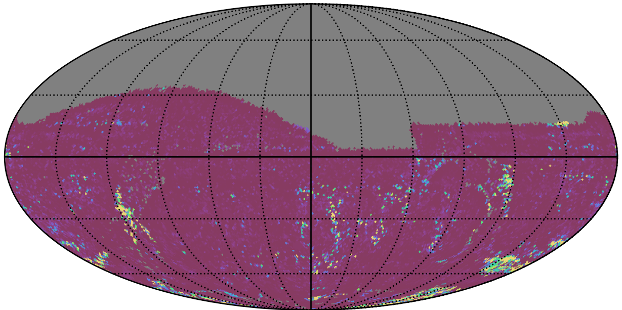
weather_cloudso2v3.4_10yrs All sky g band: 75th Percentile Intranight Timespan
