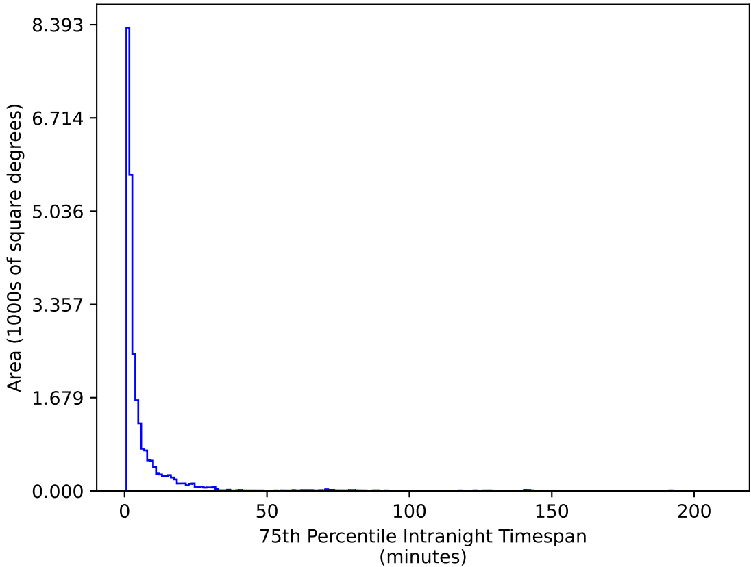
weather_cloudso2v3.4_10yrs All sky g band: 75th Percentile Intranight Timespan
