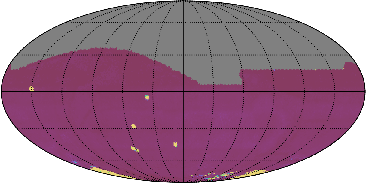
weather_cloudso2v3.4_10yrs All sky all bands: 75th Percentile Intranight Timespan
