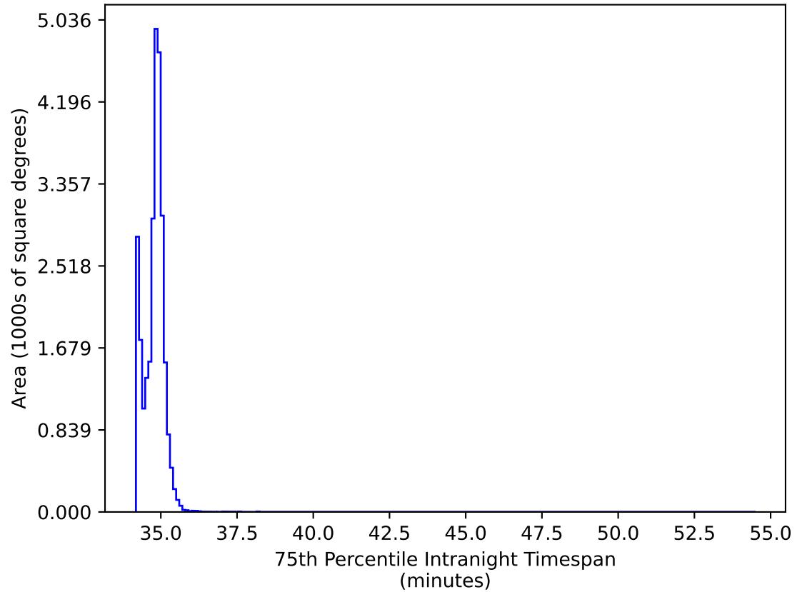
weather_cloudso2v3.4_10yrs All sky all bands: 75th Percentile Intranight Timespan
