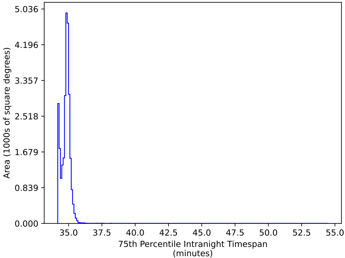
weather_cloudso2v3.4_10yrs All sky: 75th Percentile Intranight Timespan
