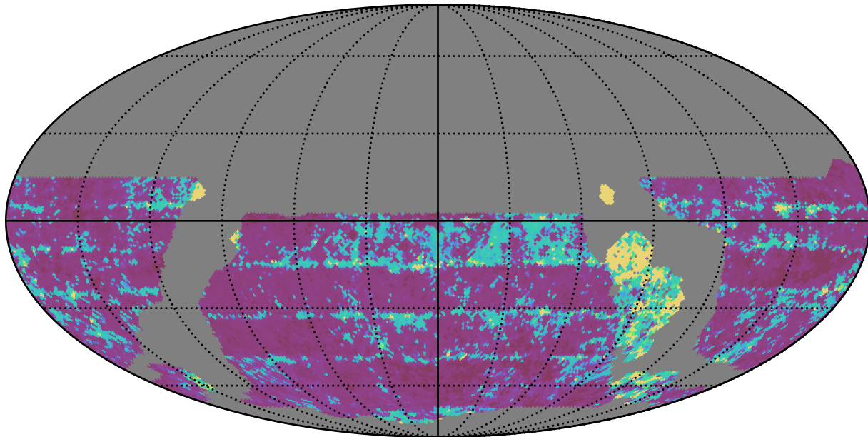
weather_cloudso2v3.4_10yrs WFD z band: 20thPercentile Inter-Night Gap
