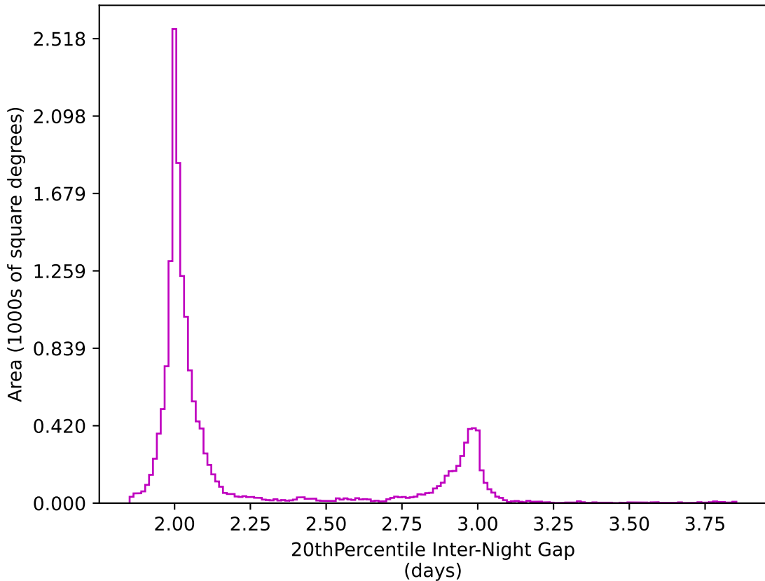
weather_cloudso2v3.4_10yrs WFD z band: 20thPercentile Inter-Night Gap
