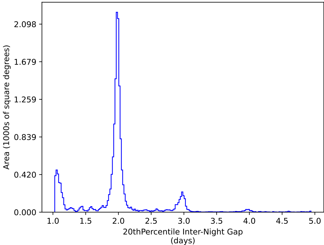
weather_cloudso2v3.4_10yrs WFD y band: 20thPercentile Inter-Night Gap
