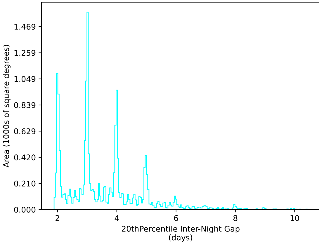
weather_cloudso2v3.4_10yrs WFD u band: 20thPercentile Inter-Night Gap
