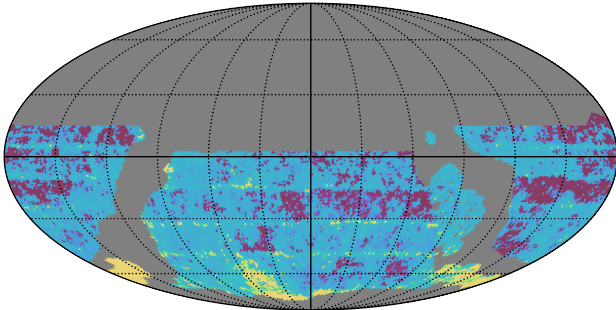
weather_cloudso2v3.4_10yrs WFD r band: 20thPercentile Inter-Night Gap
