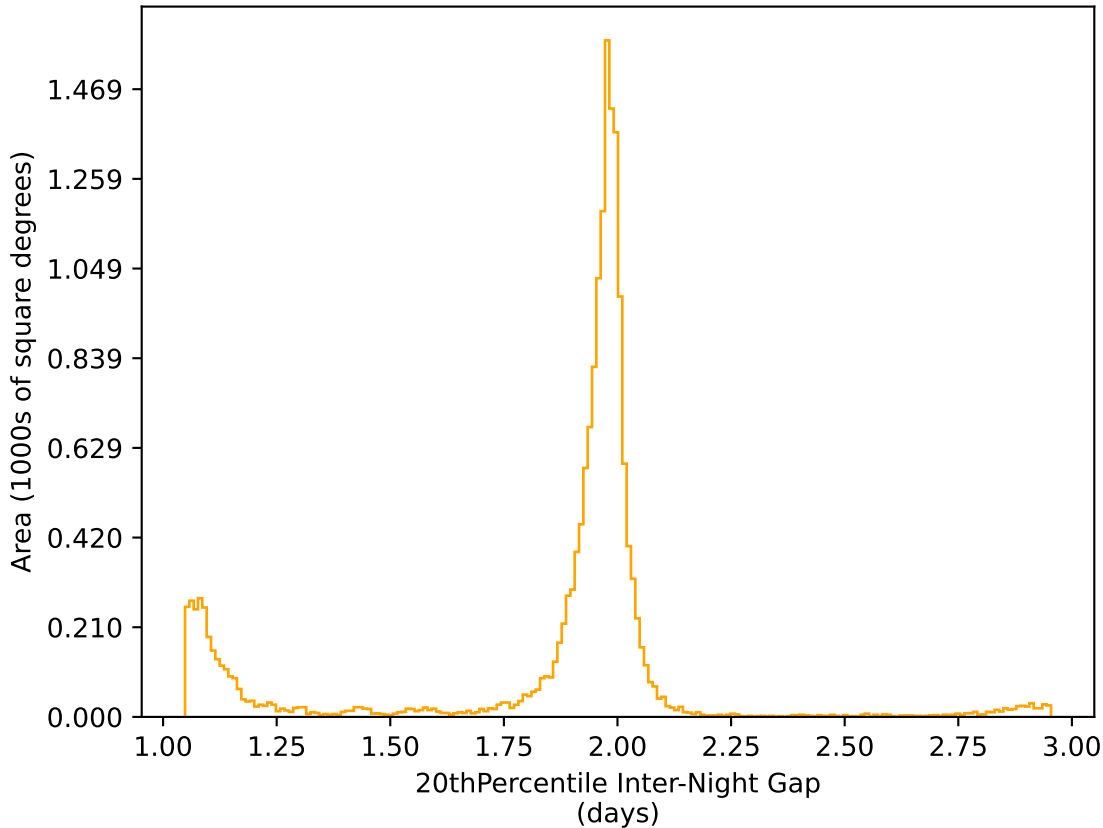
weather_cloudso2v3.4_10yrs WFD r band: 20thPercentile Inter-Night Gap
