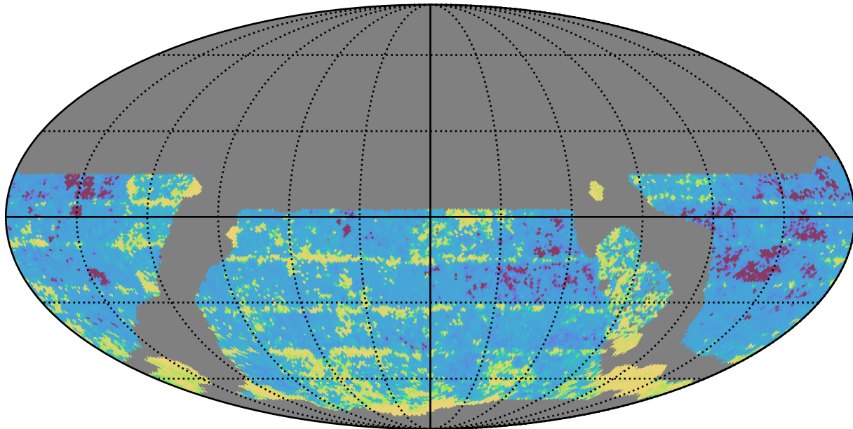
weather_cloudso2v3.4_10yrs WFD i band: 20thPercentile Inter-Night Gap
