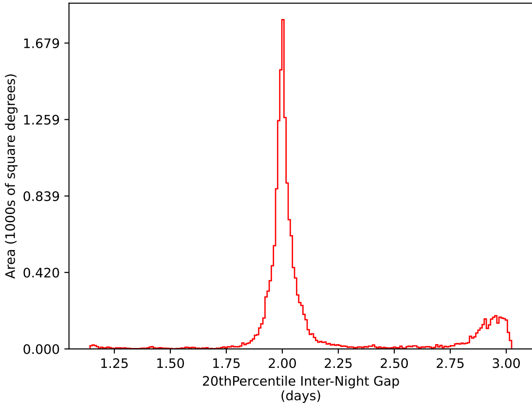
weather_cloudso2v3.4_10yrs WFD i band: 20thPercentile Inter-Night Gap
