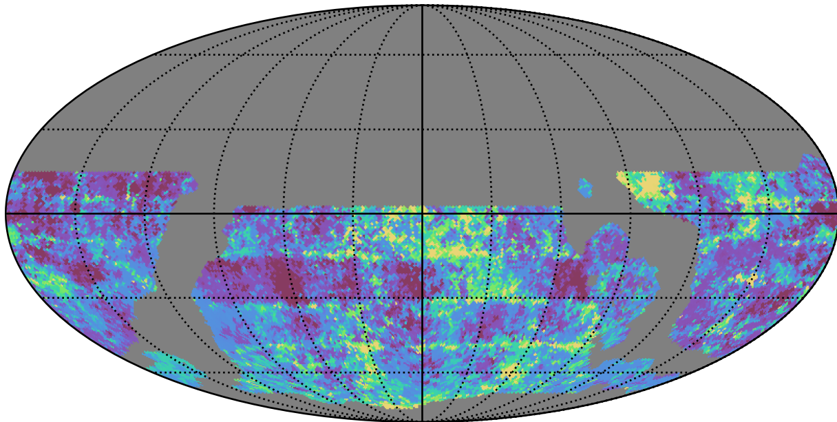
weather_cloudso2v3.4_10yrs WFD g band: 20thPercentile Inter-Night Gap
