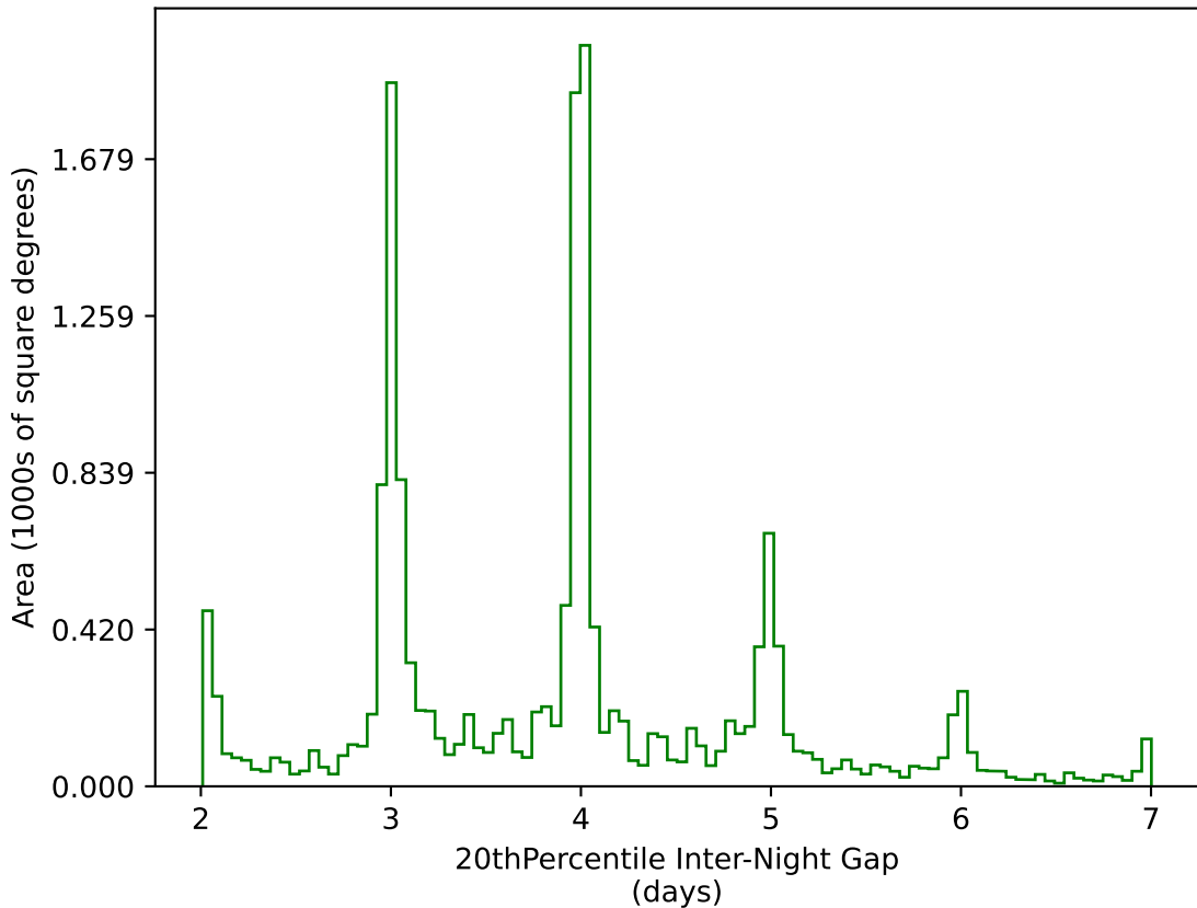
weather_cloudso2v3.4_10yrs WFD g band: 20thPercentile Inter-Night Gap
