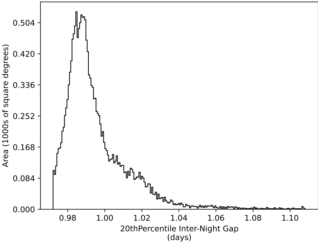
weather_cloudso2v3.4_10yrs WFD all bands: 20thPercentile Inter-Night Gap
