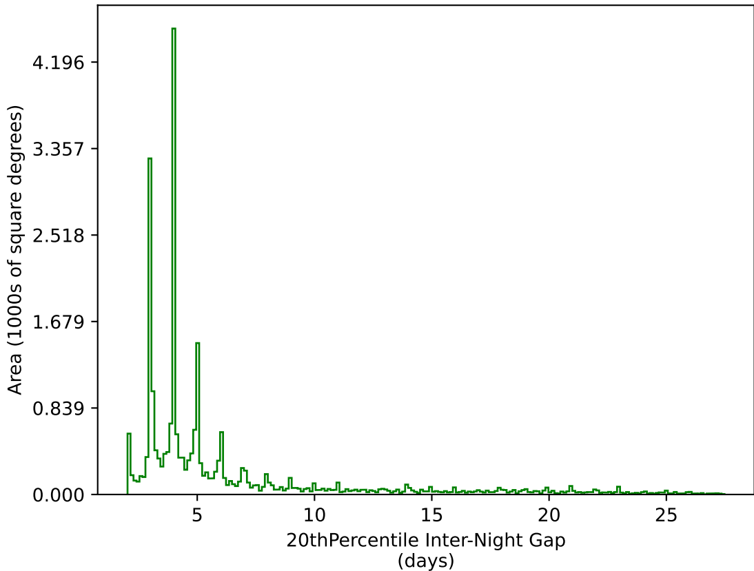
weather_cloudso2v3.4_10yrs All sky g band: 20thPercentile Inter-Night Gap
