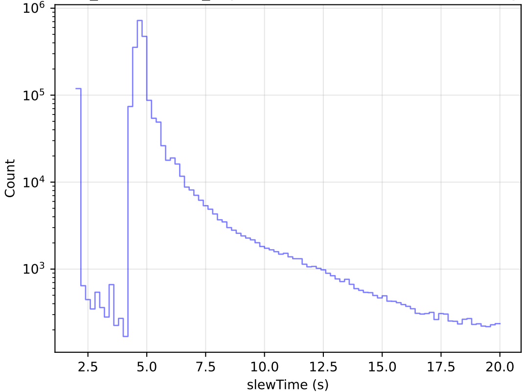
weather_cloudso2v3.4_10yrs All visits: Zoom Slew Time Histogram
