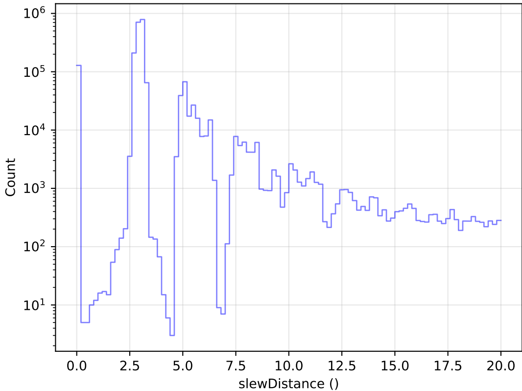
weather_cloudso2v3.4_10yrs All visits: Zoom Slew Distance Histogram
