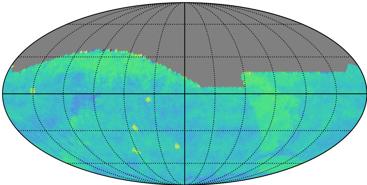
weather_cloudso2v3.4_10yrs (g or r or i): PairFraction
