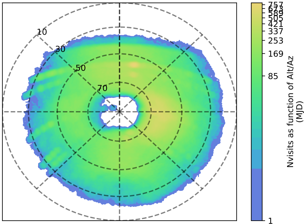
weather_cloudso2v3.4_10yrs u: Nvisits as function of Alt/Az
