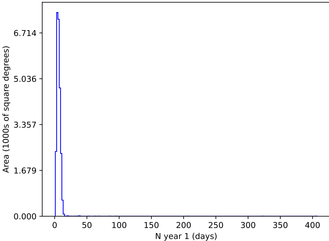
weather_cloudso2v3.4_10yrs u and night < 365: N year 1
