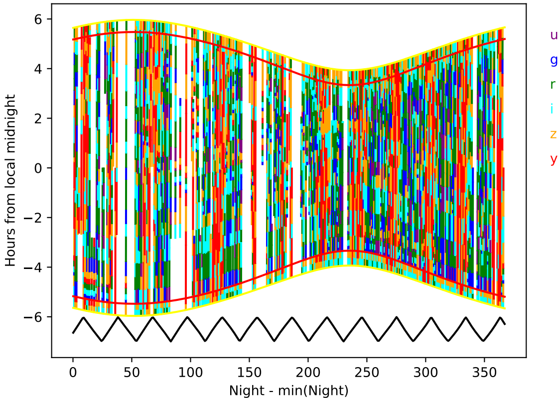
weather_cloudso2v3.4_10yrs year 3-4: Hourglass
