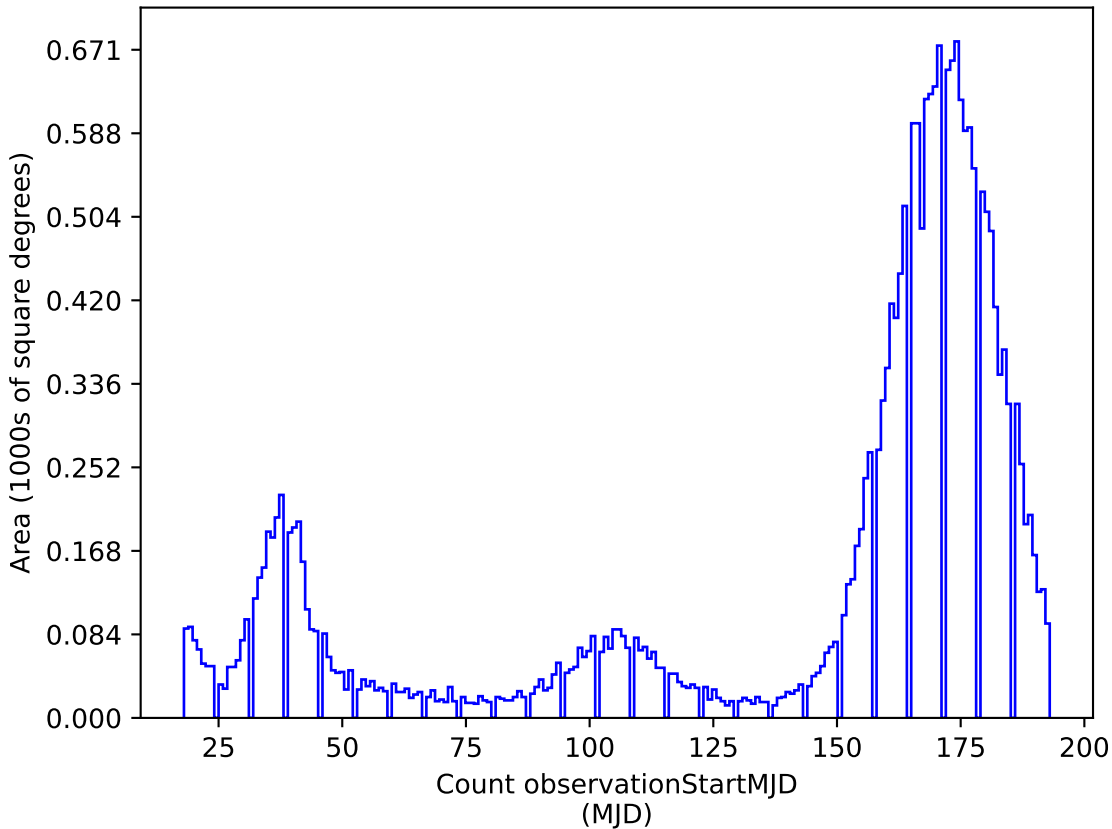
weather_cloudso2v3.4_10yrs y: Count observationStartMJD
