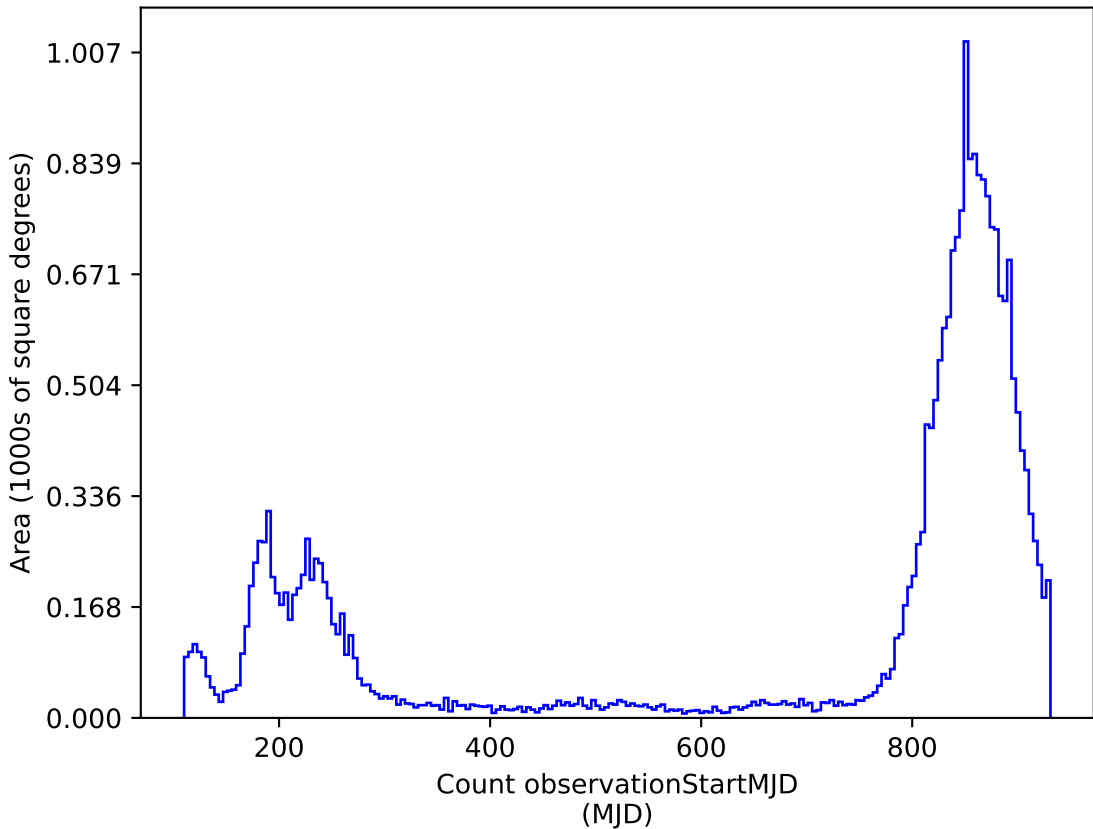
weather_cloudso2v3.4_10yrs : Count observationStartMJD
