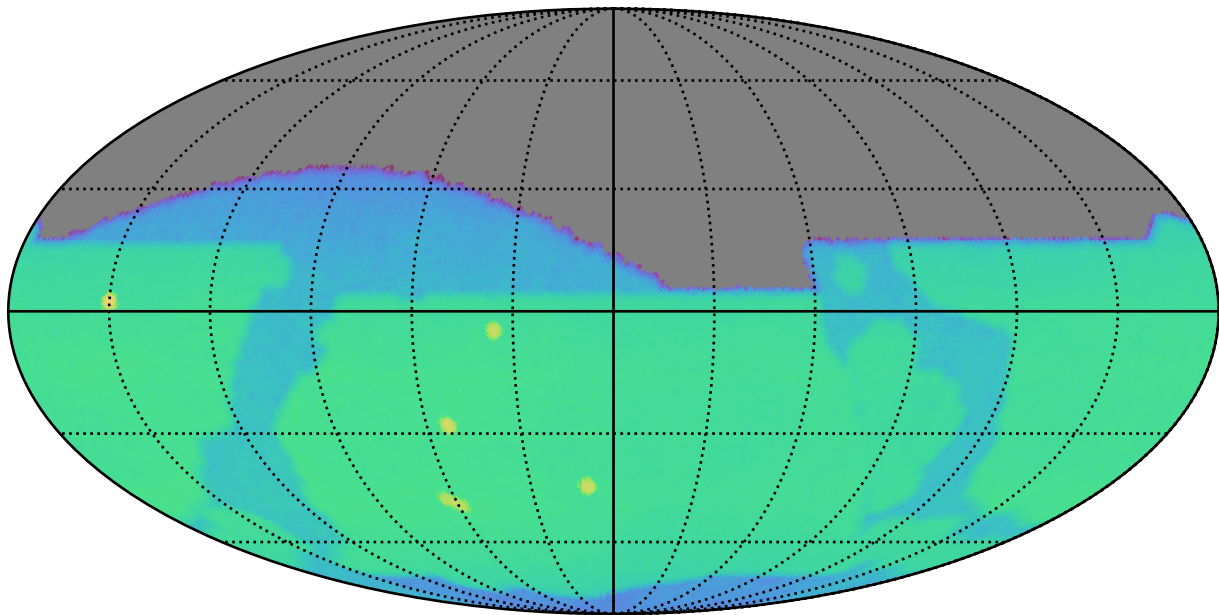
weather_cloudso2v3.4_10yrs z: CoaddM5
