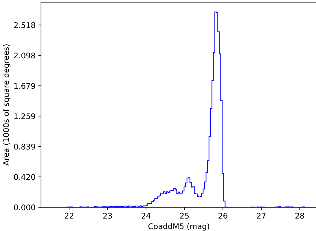
weather_cloudso2v3.4_10yrs z: CoaddM5
