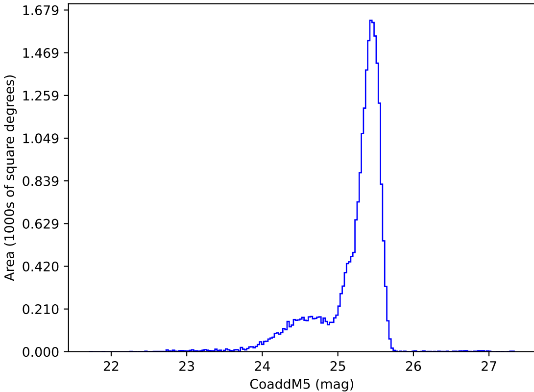
weather_cloudso2v3.4_10yrs u: CoaddM5
