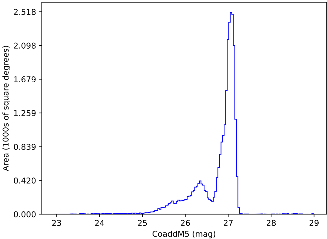
weather_cloudso2v3.4_10yrs r: CoaddM5
