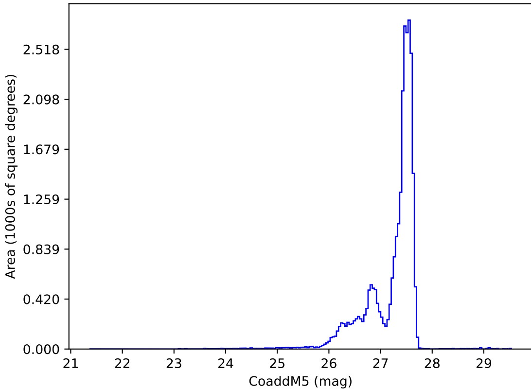
weather_cloudso2v3.4_10yrs : CoaddM5
