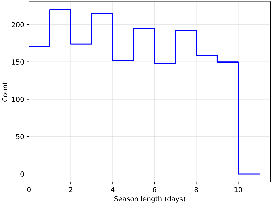
weather_cloudso2v3.4_10yrs DD:WFD all bands: SeasonLength
