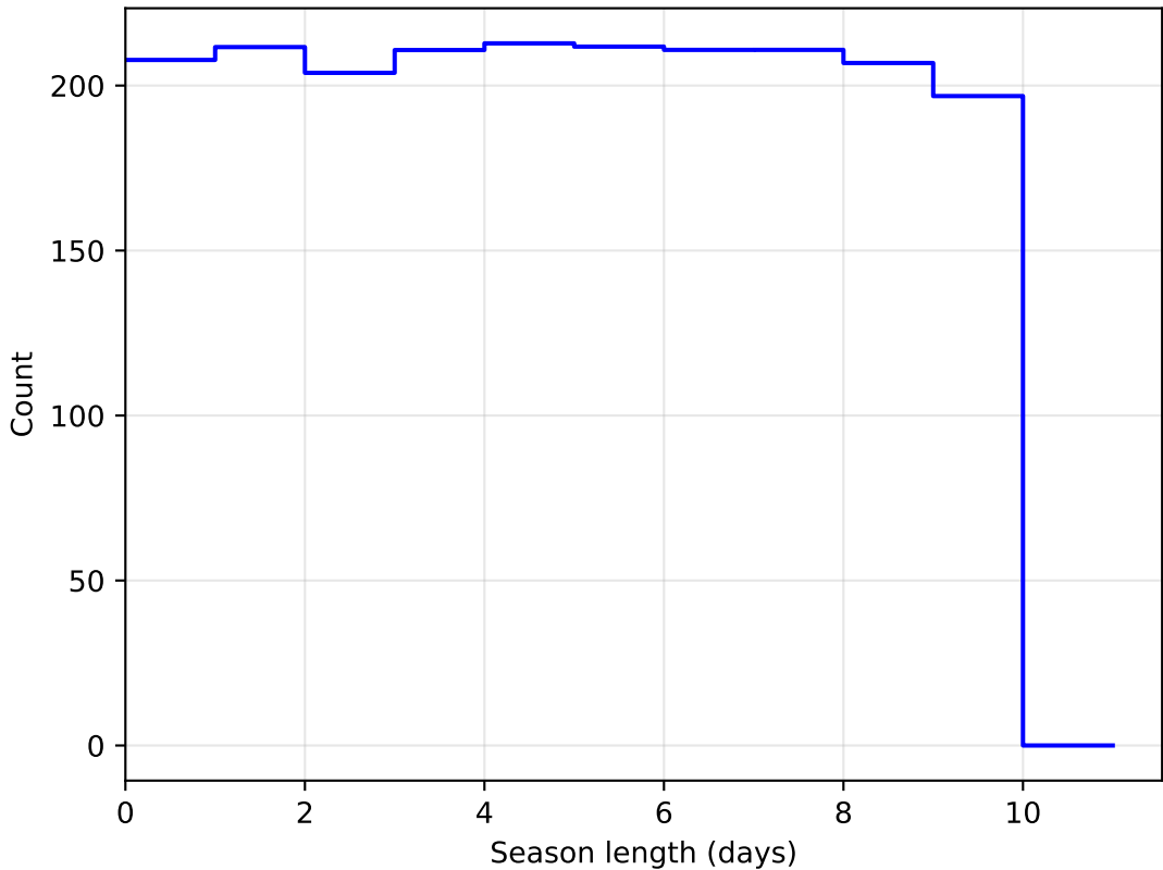
weather_cloudso2v3.4_10yrs DD:EDFS all bands: SeasonLength
