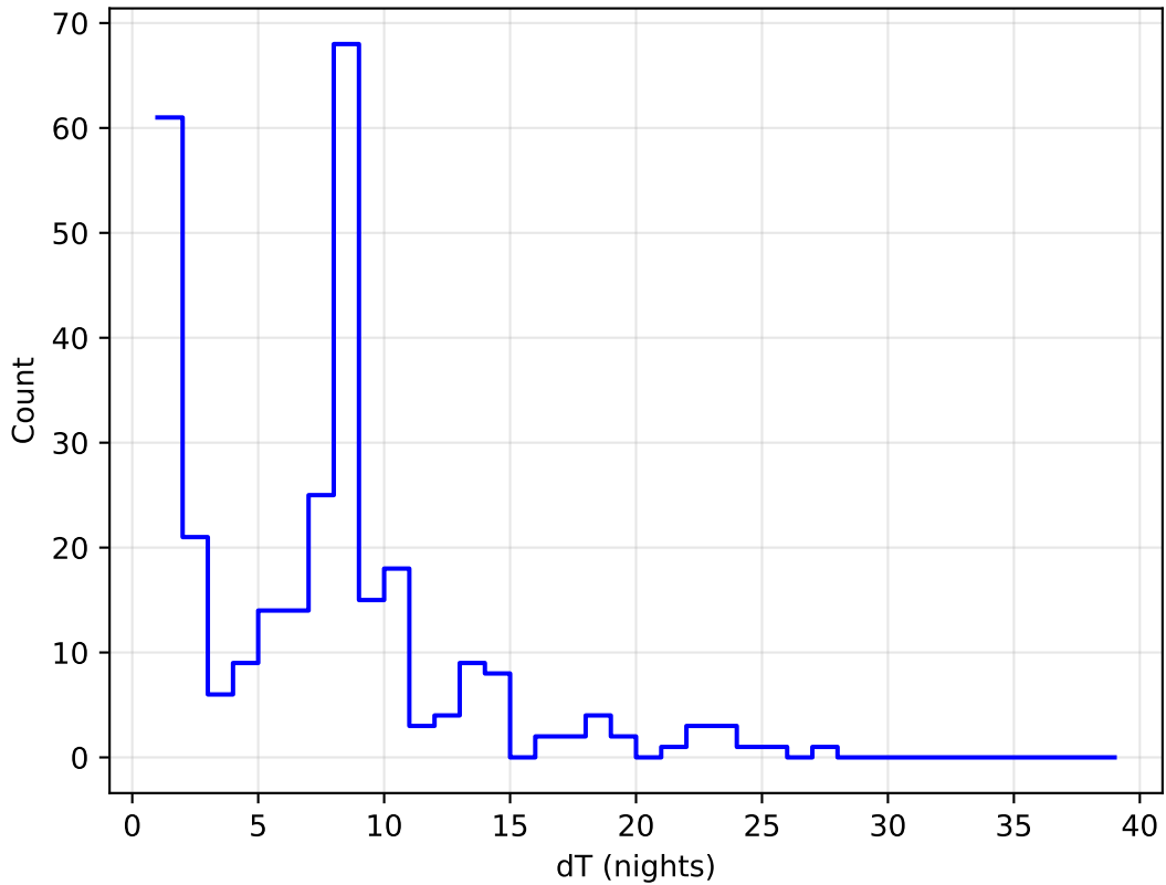
weather_cloudso2v3.4_10yrs all bands: DD:XMM_LSS Delta Nights Histogram
