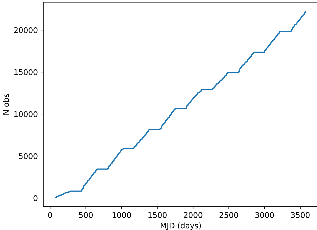
weather_cloudso2v3.4_10yrs all bands: DD:XMM_LSS Cumulative NVisits
