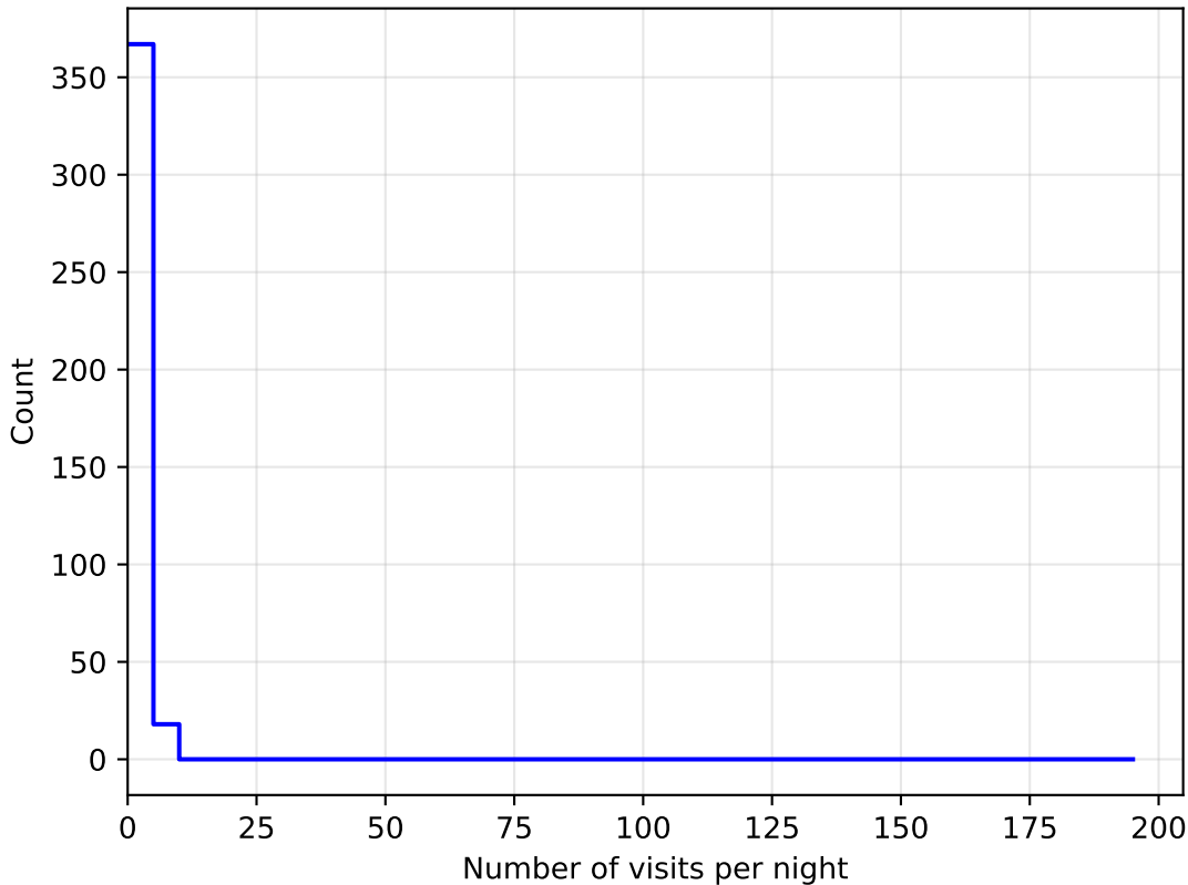
weather_cloudso2v3.4_10yrs all bands: DD:WFD NVisitsPerNight
