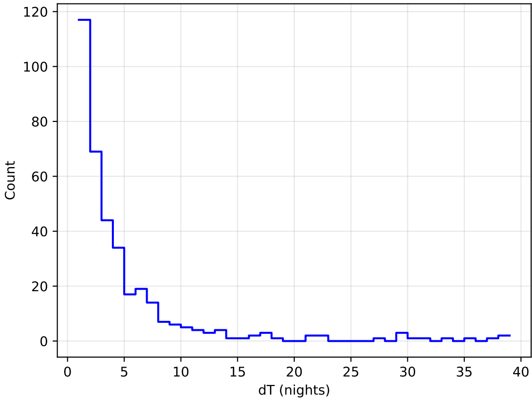
weather_cloudso2v3.4_10yrs all bands: DD:WFD Delta Nights Histogram
