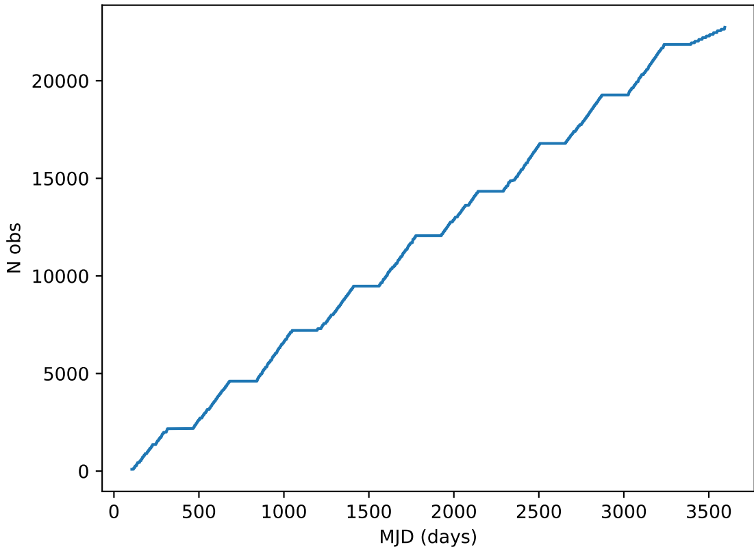
weather_cloudso2v3.4_10yrs all bands: DD:EDFS Cumulative NVisits
