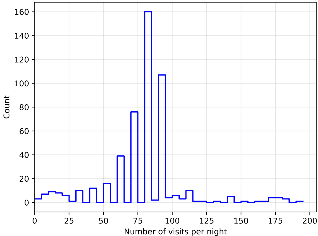
weather_cloudso2v3.4_10yrs all bands: DD: COSMOS NVisitsPerNight
