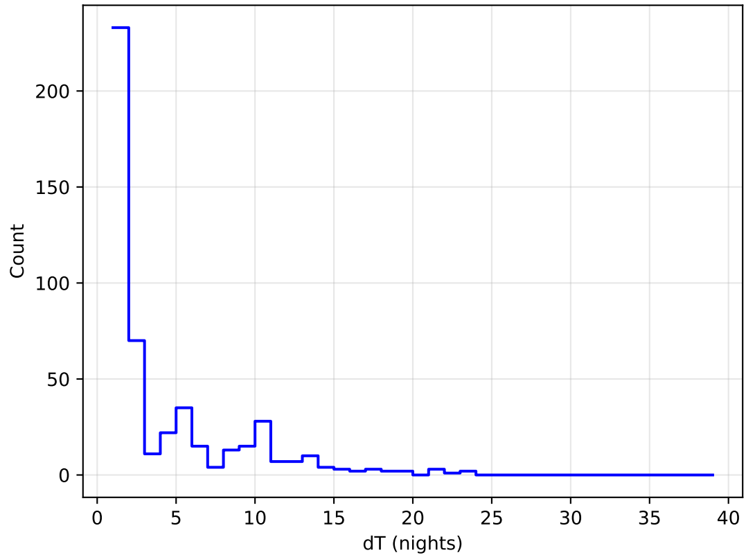
weather_cloudso2v3.4_10yrs all bands: DD: COSMOS Delta Nights Histogram
