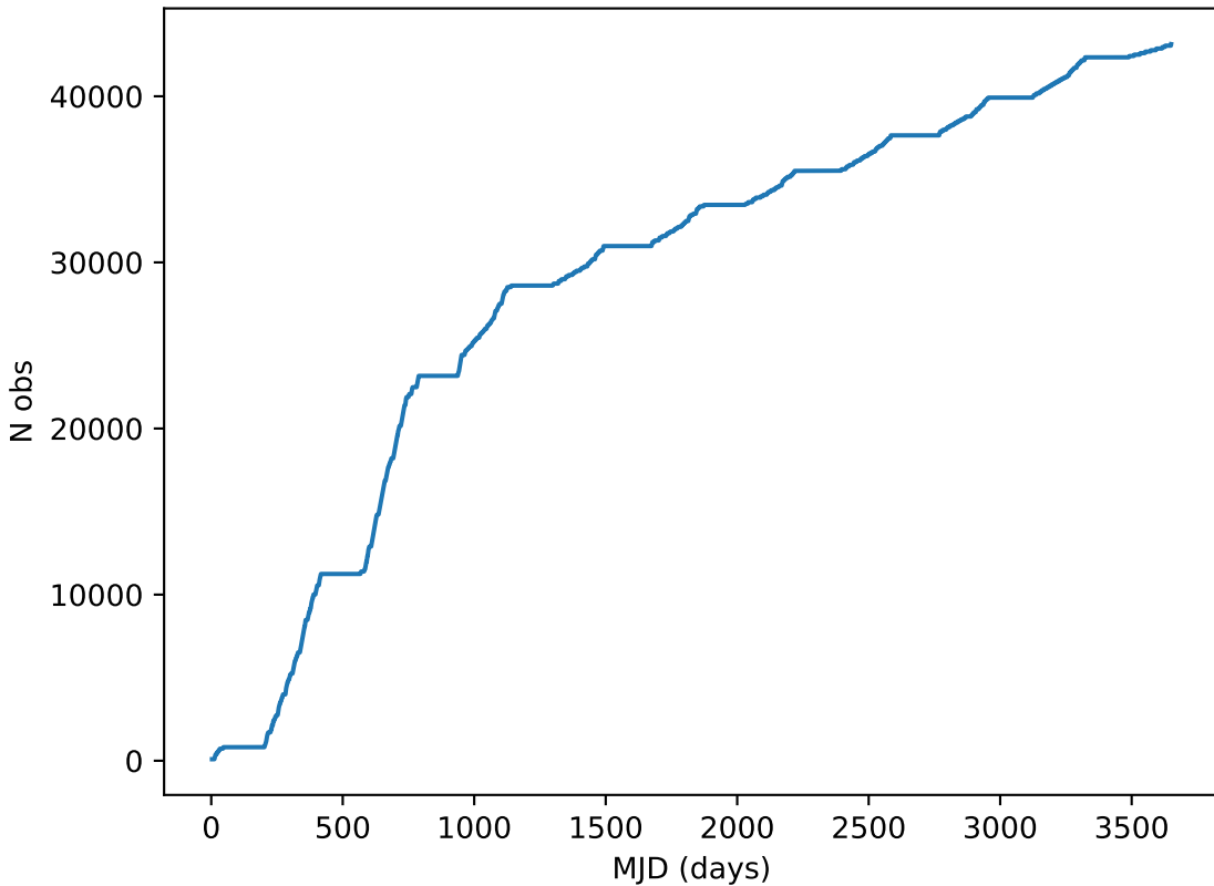
weather_cloudso2v3.4_10yrs all bands: DD:COSMOS Cumulative NVisits
