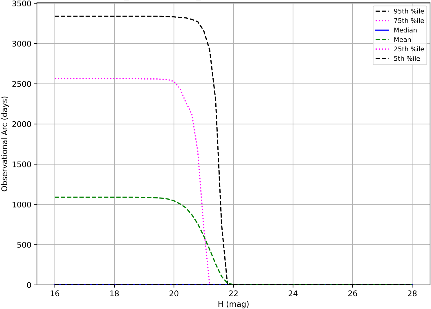
weather_cloudso20v3.4_10yrs: Observational Arc Length Vatra
