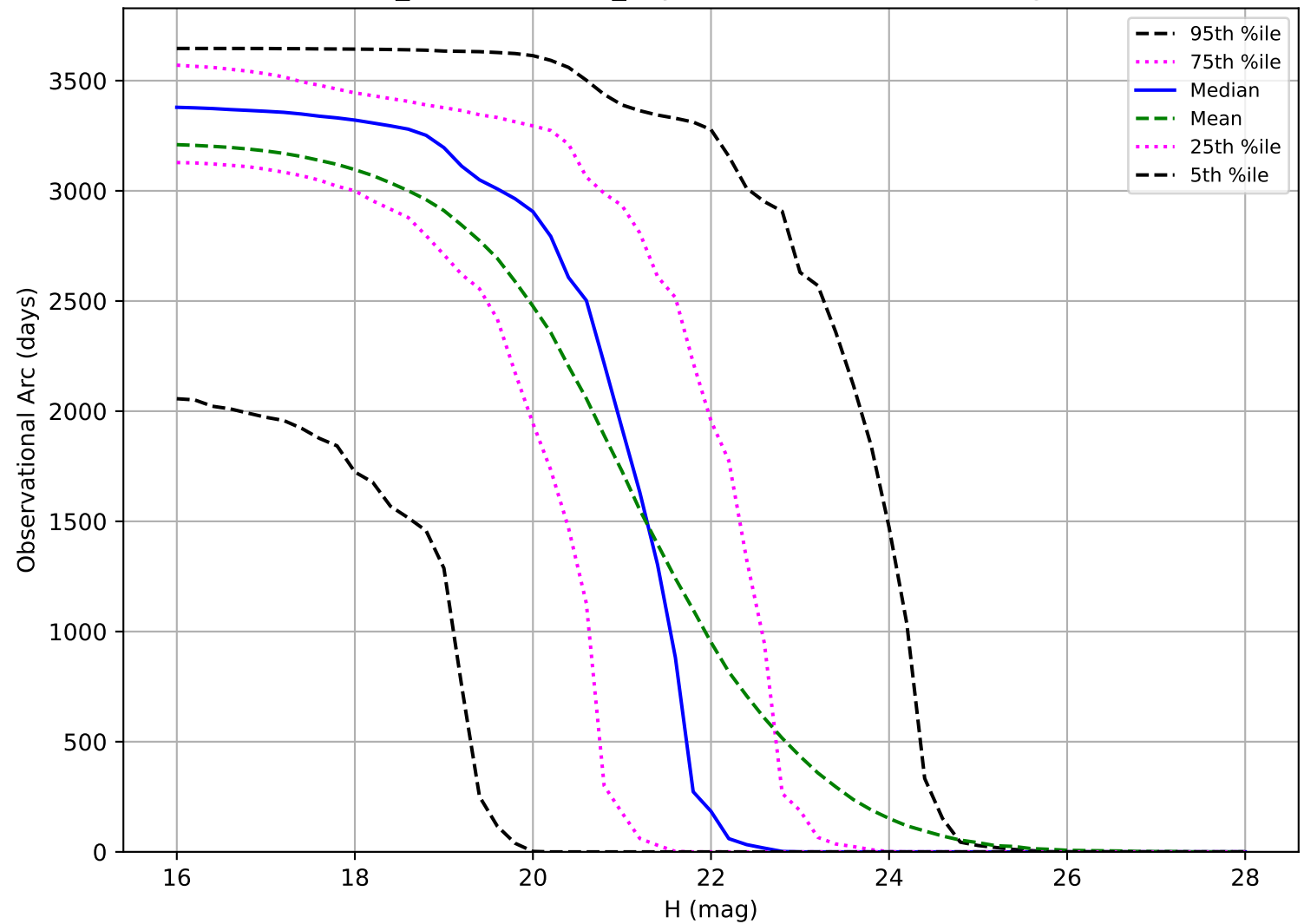
weather_cloudso20v3.4_10yrs: Observational Arc Length PHA
